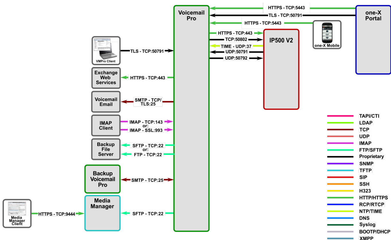
Voicemail Pro Port Usage
